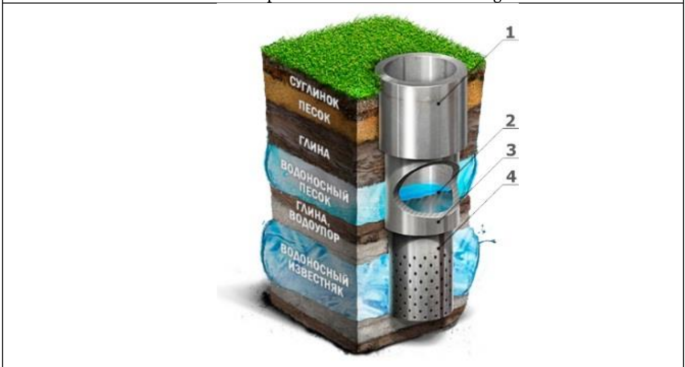
Drilling a well for technical water on the territory of the university.
