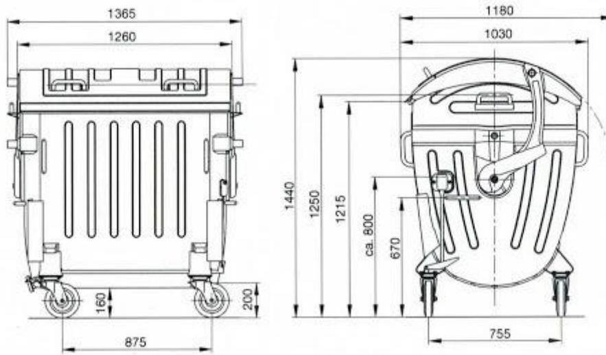
Schematic representation of a galvanized waste container
